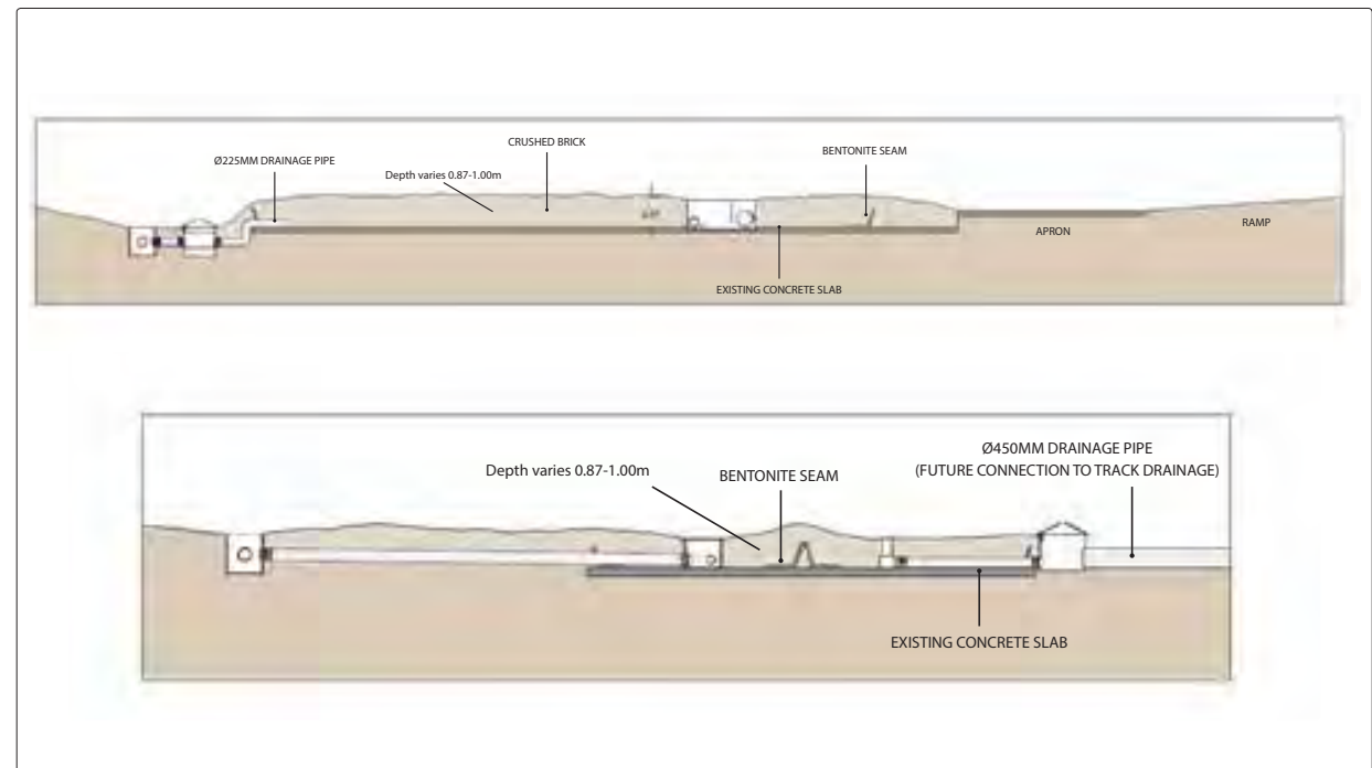
Swale sections
