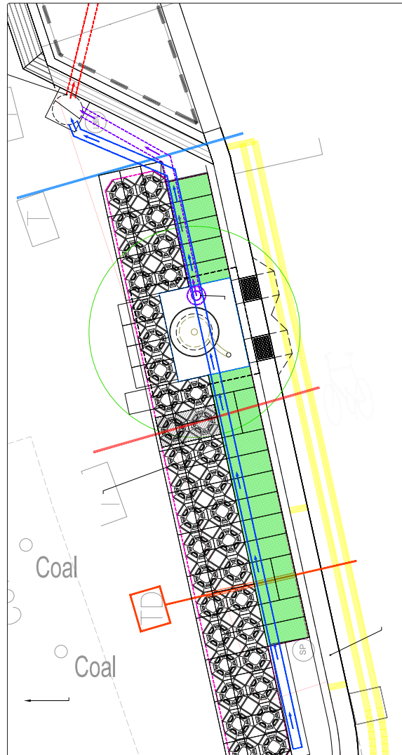
Plan showing modular soil system
