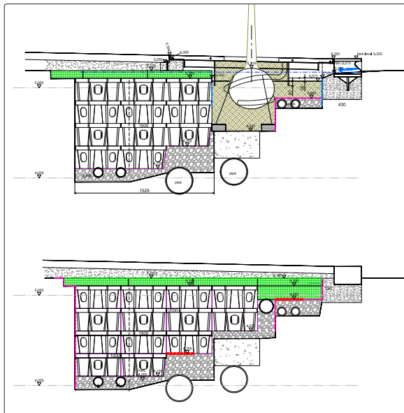
Tree pit details
